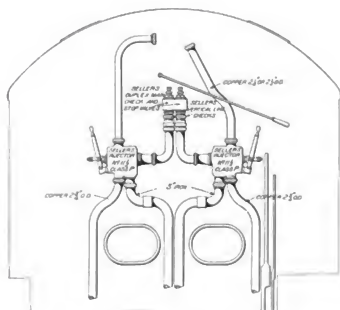
Fig. 3109. Arrangement of Injectors on Back Head of Boiler of Atlantic (4-1-2) Locomotive. P. R. R.
